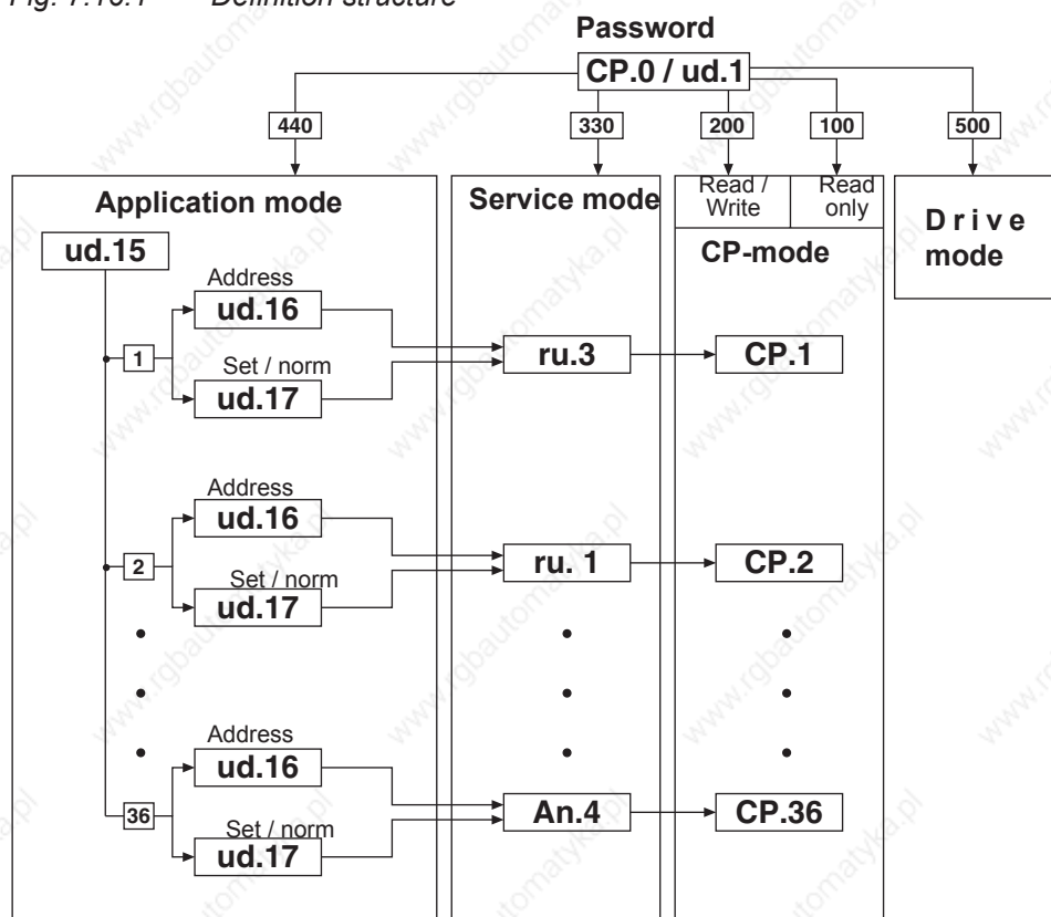
Fig. 7.16.1 Definition structure
