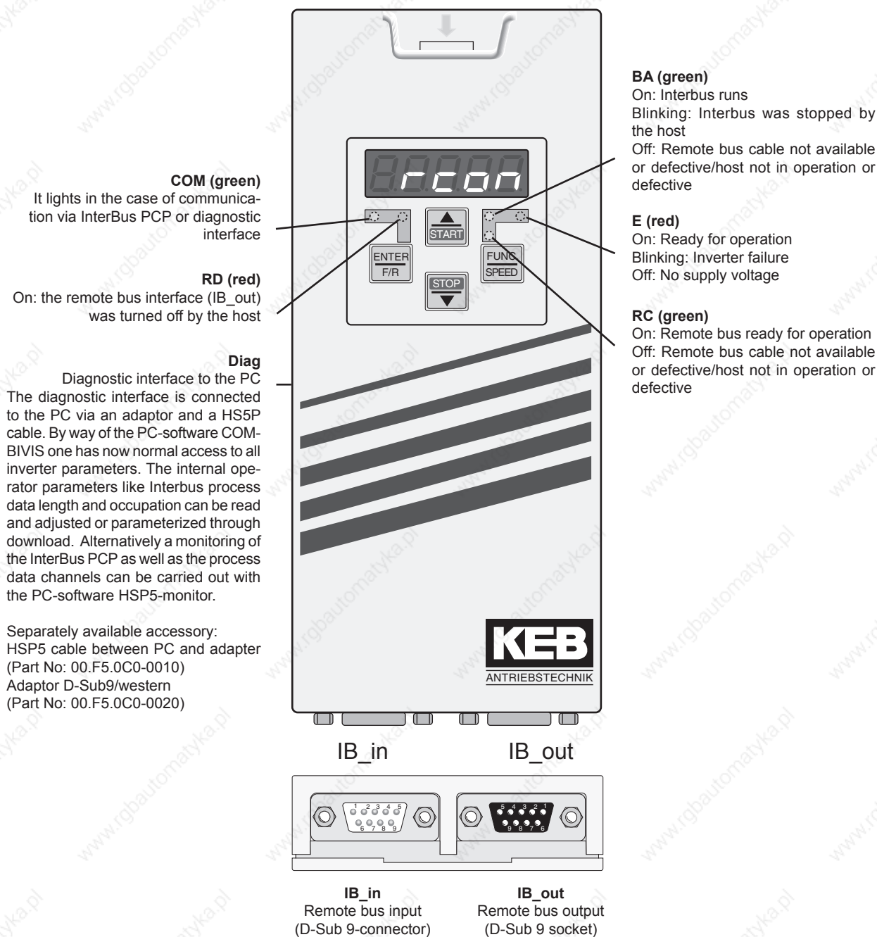
Fig. 11.1.6 InterBus operator
