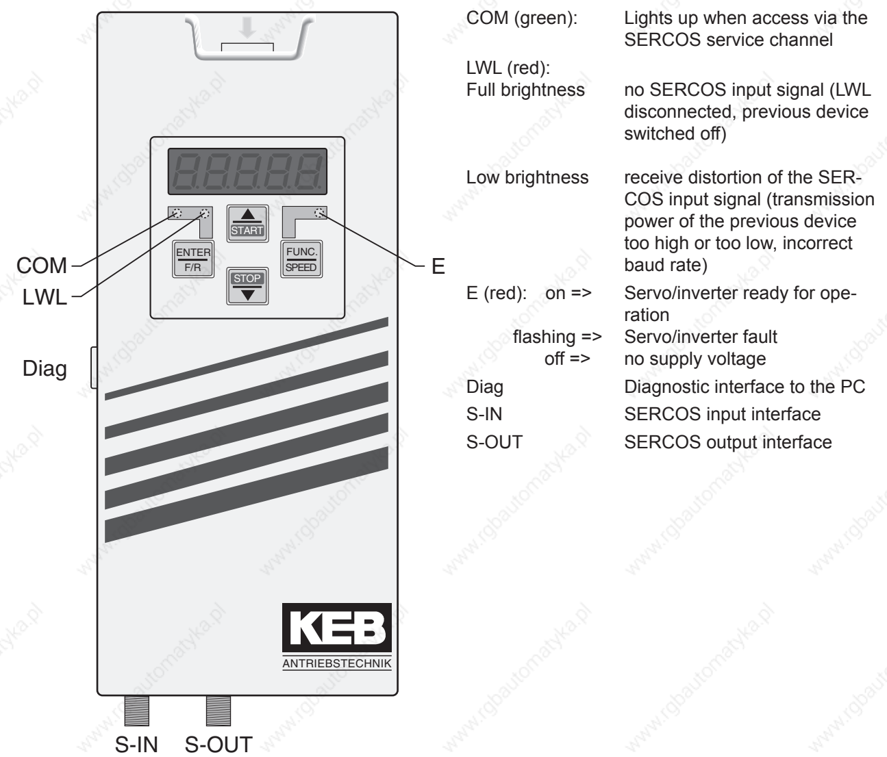
Fig. 11.1.8 Sercos operator
